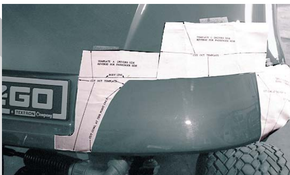
STEP 3: Align template C with templates A & B and 1/8" below the body line as shown above.
