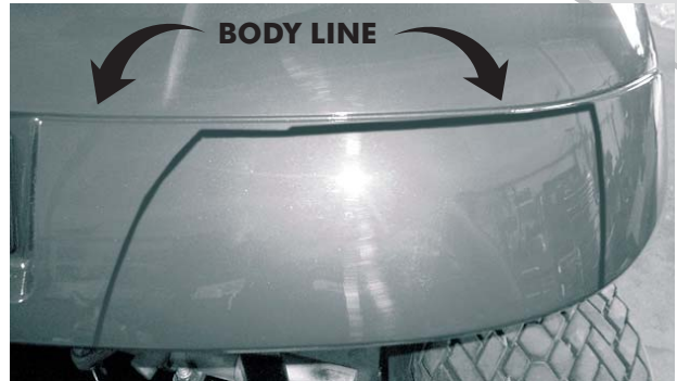
STEP 4: With all of the templates in place take a black marker and outline (follow along) outer edge of the templates. CUT 1/8" BELOW THE BODY LINE. DO NOT CUT AT OR ABOVE BODY LINE.
