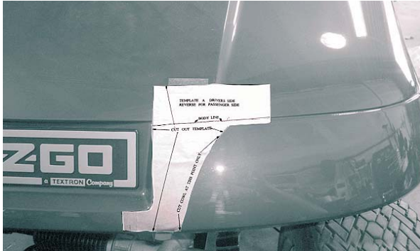
STEP 1: Align template A with body line - Front.
